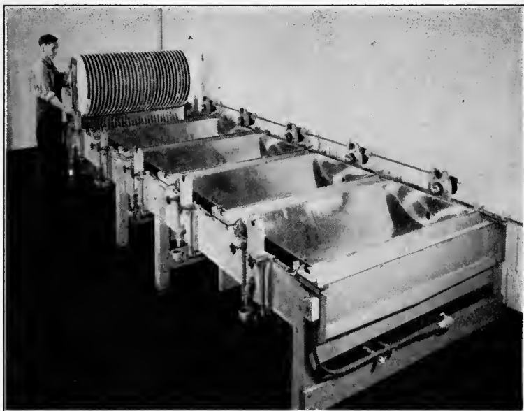
FIG. 1. The complete developing machine.
